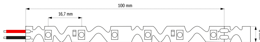
SMD 2835
